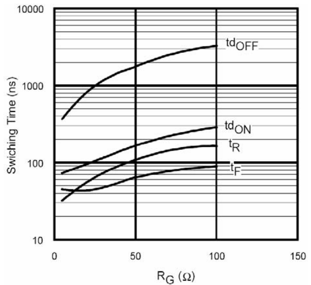
Fig 12. Typ. Switching Time vs. R g T J = 125°C; L = 200μH; V CE = 600V I CE = 150A; V GE = 15V
