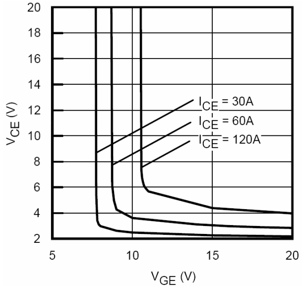
Fig 8. Typical V_{CE} vs. V_{GE} T_J = 125^\circ\text{C}
